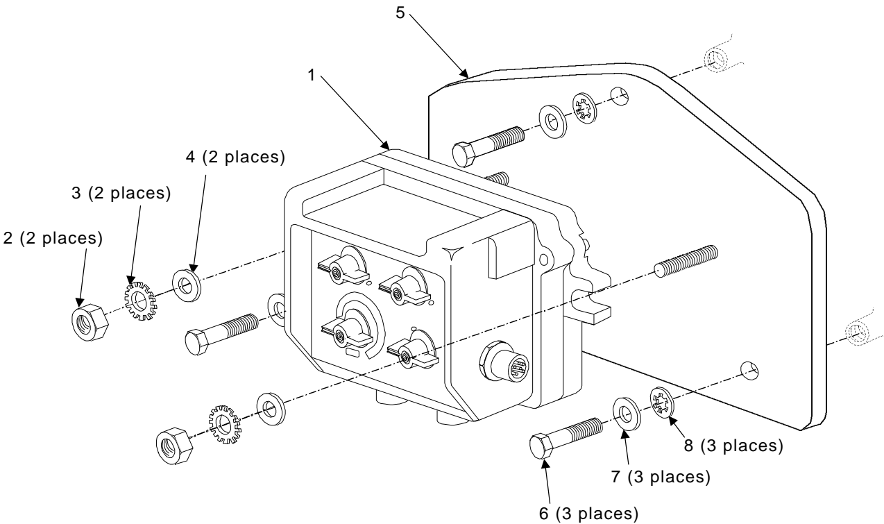
Figure 4-4. Commander's FFCS Installation
