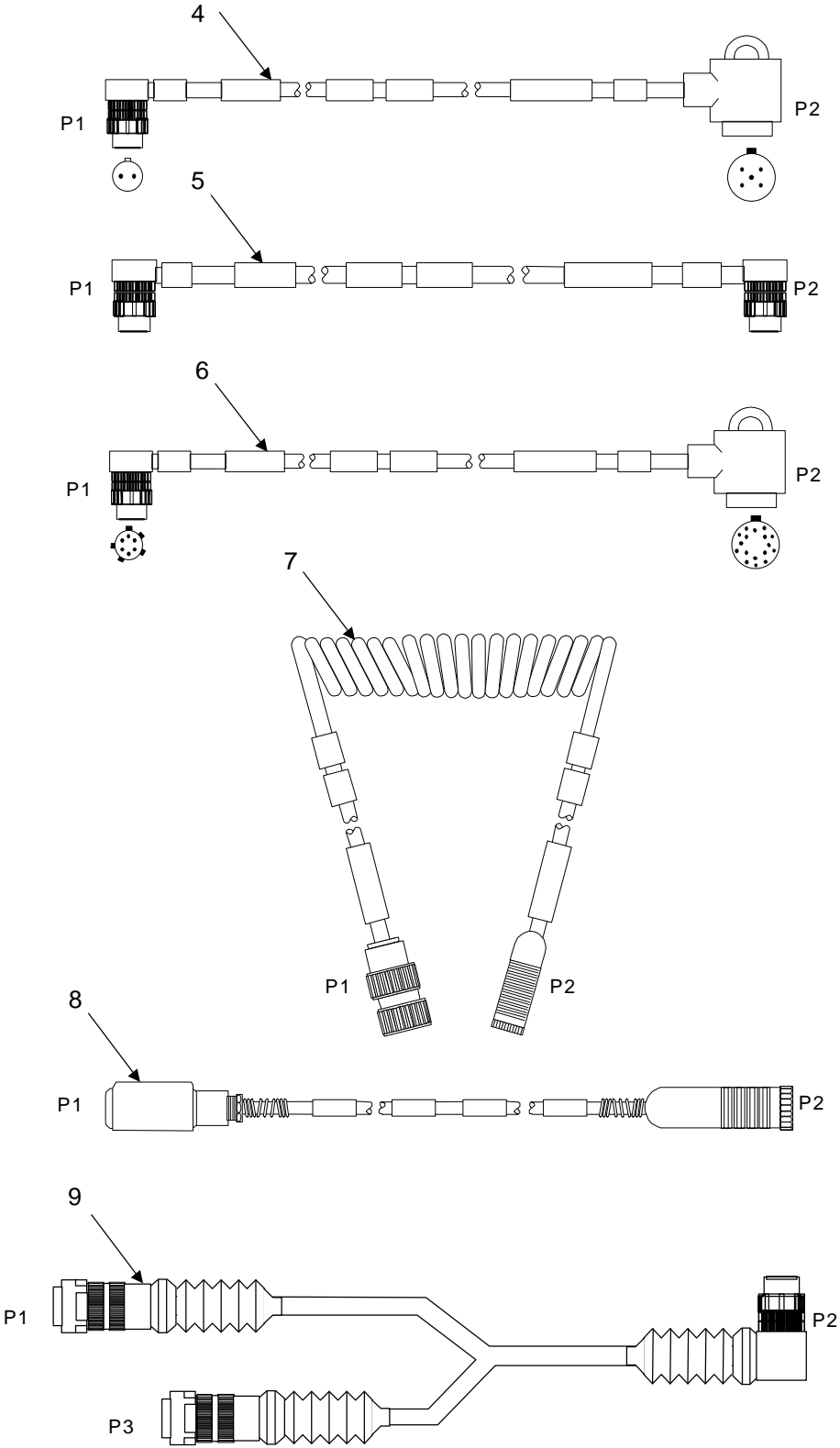
Figure 2-2. Illustrated Parts List - Cables
