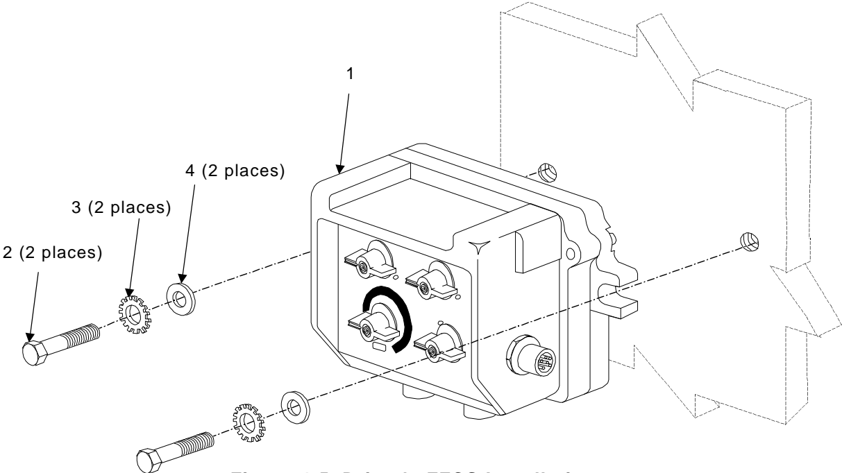
Figure 4-5. Driver's FFCS Installation
